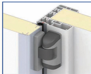
Connecting Door to the Frame
